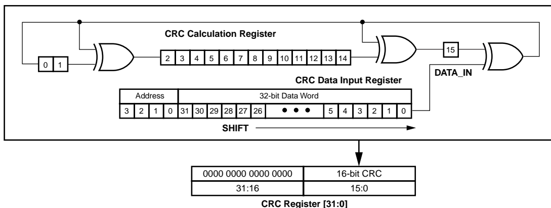
Figure 12: Serial 16-bit CRC Circuitry
